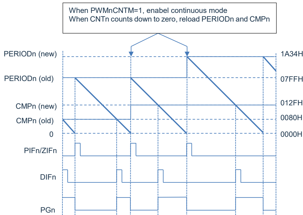
Figure 13-1: edge-aligned timing diagram
